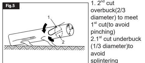
Figure 5 – Log supported one end 1. 2 nd cut overbuck(2/3 diameter) to meet 1 st cut(to avoid pinching) 2. 1 st cut underbuck (1/3 diameter)to avoid splintering
