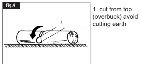
Figure 4 – Log supported along the entire length 1. cut from top (overbuck) avoid cutting earth
